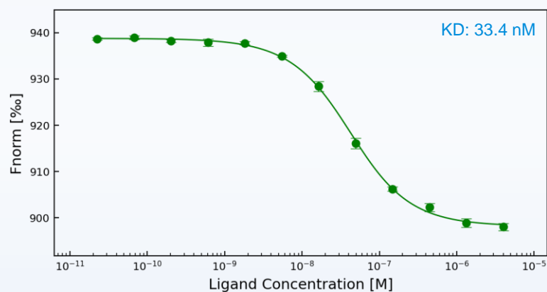
Ternary complex formation: CRBN-DDB1 + CC-885 vs. GSPT1
