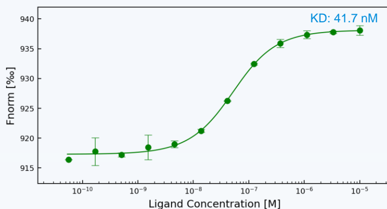
Ternary complex formation: CRBN-DDB1 + CC-885 vs. GSPT1
