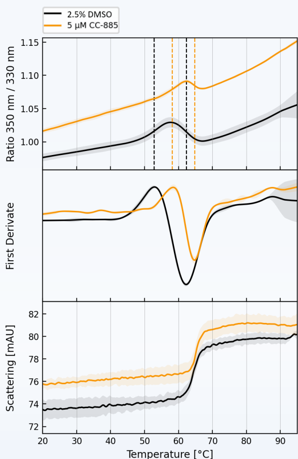
Ternary complex formation: CRBN-DDB1 + CC-885 vs. GSPT1
