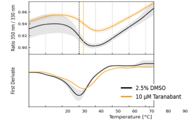
nanoDSF: CNR1 vs Taranabant
