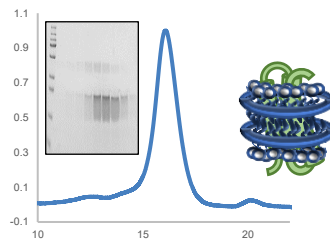
G-protein: Gai-β-γ
