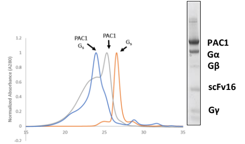
PAC1-Gs complex
