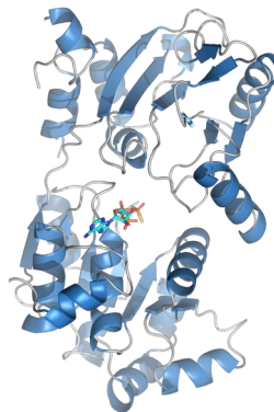
ATPγS bound
